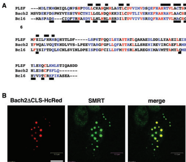
Fig. 1. Comparison of BTB domains among three BTB-type repressors. (A) N-terminal 130 amino acids in BTB domains of Bach2, Bcl6 and PLZF were aligned with a clustalw software. Upper and under lines represent important residues for interaction with SMRT (11, 19). (B) The Bach2 focus contains endogenous SMRT. MCF7 cells were transfected with Bach2ΔCLS-HcRed and EGFP-HDAC4ΔNES expression vectors. Endogenous SMRT was stained with an anti-SMRT antibody. A scale bar in the left panel indicates 10 μm.
