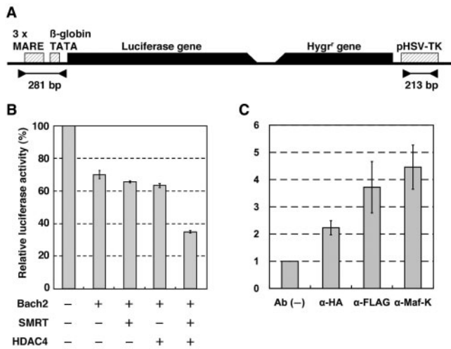
Fig. 7. Effect of Bach2 focus formation on MARE regulated transcription. (A) A schematic diagram of the reporter plasmid introduced into the RBGP2 cell lines. The TK promoter has no MARE sequence. Black triangles and lines represent PCR primers for the ChIP experiment and the putative PCR products, respectively. (B) Relative transcription activity. The RBGP2 cells were transiently transfected with the expression plasmids with several combinations, and then the luciferase activity was measured. (C) ChIP analysis. The RBGP2 cells were co-transfected with expression plasmids for Bach2, HA-SMRT 1205-1668 and HDAC4-FLAG. ChIP experiments were performed with a rabbit serum [Ab (-)], an anti-FLAG, an anti-HA or an anti-MafK antibody. Note that both SMRT and HDAC4 are unable to bind directly to any DNA sequences.
