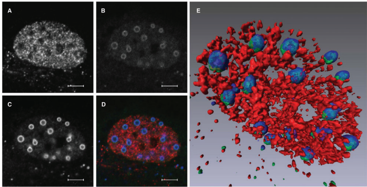
Fig. 6. Effect of Bach2 focus formation on local transcription. GM02063 cells were transiently transfected with expression plasmids for Bach2, HDAC4-FLAG and HA-SMRT 1205-1668 . Scratch transcription labelling for 5 min with 1 mM BrUTP was carried out with the transfected cells. Transcription sites, Bach2 and HDAC4 are represented in red (A), green (B) and blue (C), respectively. (D) Bach2 (green) appears to co-localize with
