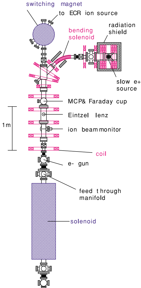
Fig. 4. Brief sketch of the beam line. The beam line is still under construction.
