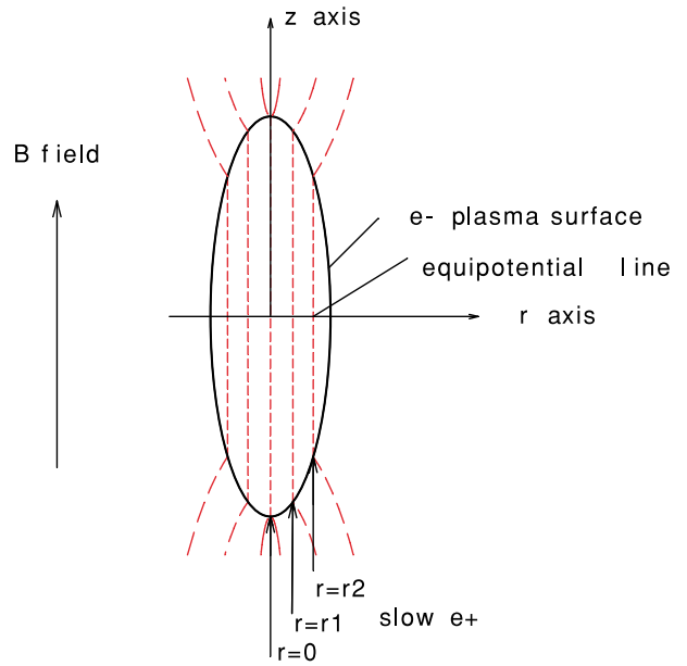
Fig. 7. Image drawing of the equipotential line in a plasma (not scaled).
