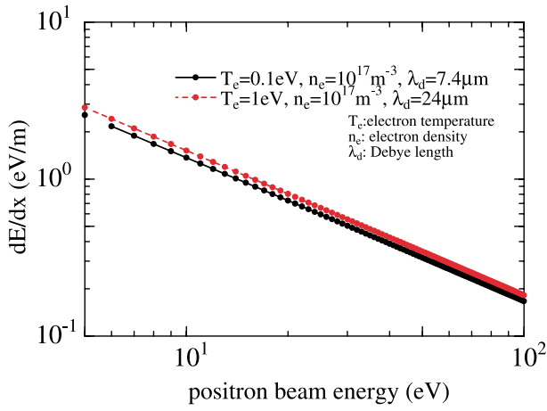
Fig. 5. Calculated positron stopping power in free electron gas. The difference parameter between two calculations are plasma temperatures, T_e = 0.1 eV, and 1 eV.
