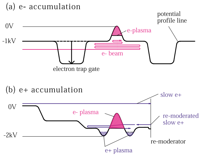
Fig. 2. Schematic view of the positron accumulation scheme using an electron plasma.
