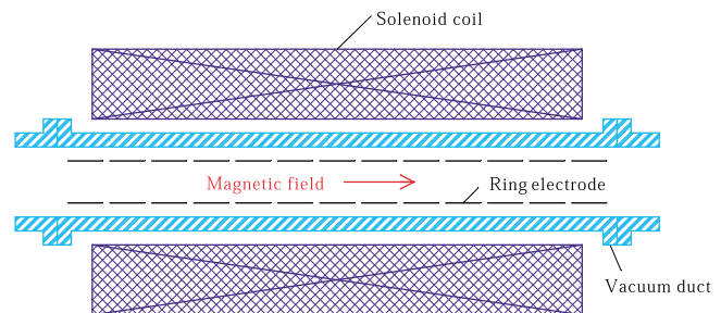
Fig. 1. Schematic drawing of the electro-magnetic trap used for positron accumulation. Charged particles can be trapped axially by an electric field and radially by a magnetic field in the trap.
