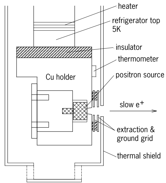
Fig. 3. Drawing of the positron source assembly.
