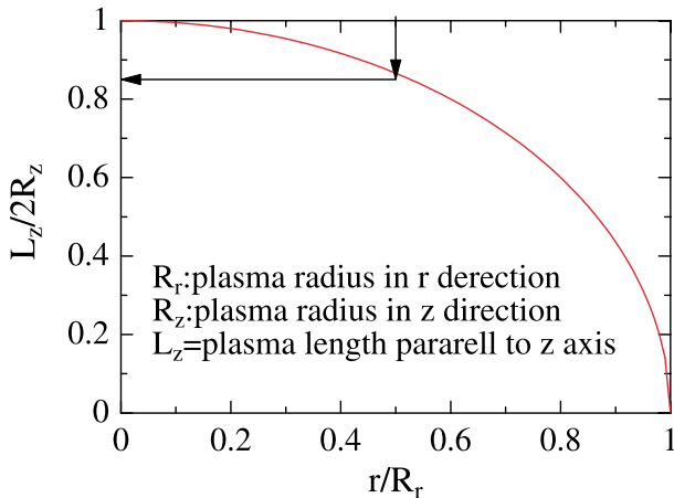
Fig. 6. Dependence of the spheroid plasma length along to z axis on r position.
