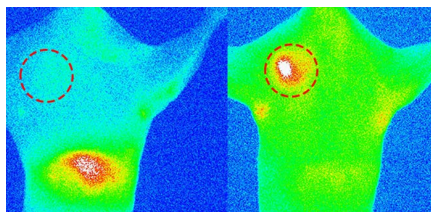
Near-infrared fluorescence images of breast tumors in mice (red circles). (left) Quantum dot injection. (right) Anti-body-conjugated quantum dots specific for breast tumor cells correctly localized to tumor area. @BDR
